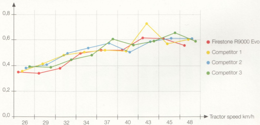
Acceleration in Z - direction in m/s 2 <
